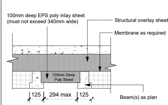
JF130 - Run-out Joint 100mm Sheet
