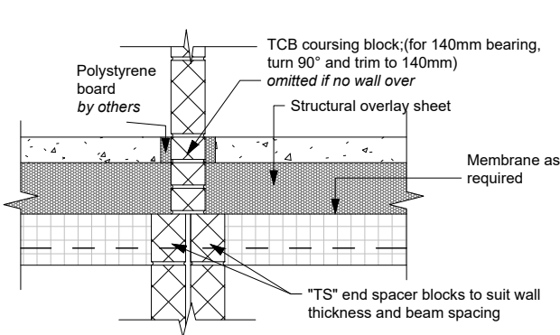
JF126 - End Bearing, min. 215mm Loadbearing Wall
