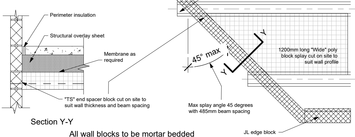
JF128 - Splayed Bearing < 45°, Wide Block
