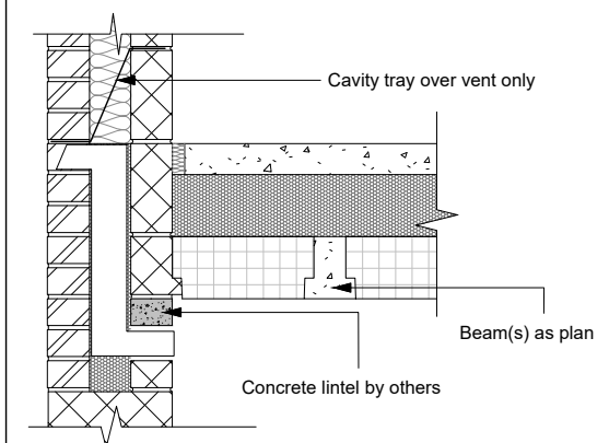
JF159 - Vent & Air Brick Detail
